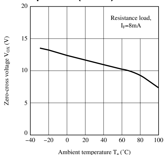
Fig.10 Zero-cross Voltage vs. Ambient Temperature (rank C)
