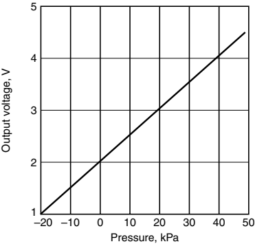
1.-(1) Output characteristics
