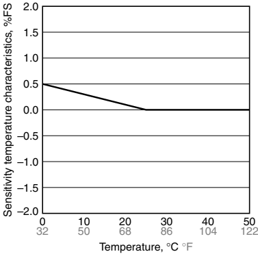
1.-(3) Sensitivity temperature characteristics
