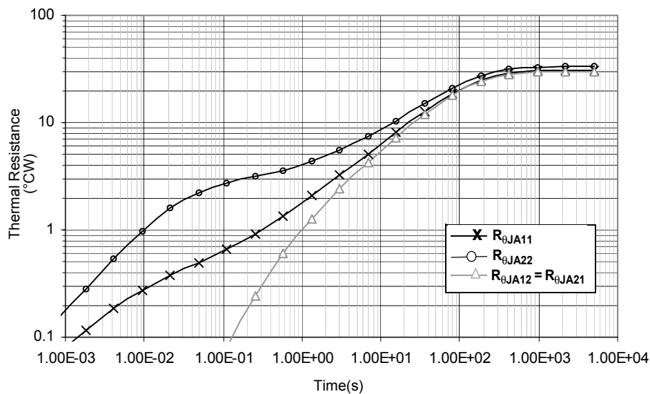
Figure 33. Transient Thermal Resistance R_{\theta JA} (1.0 W Step Response) Device on Thermal Test Board Area A = 600 (mm²)
