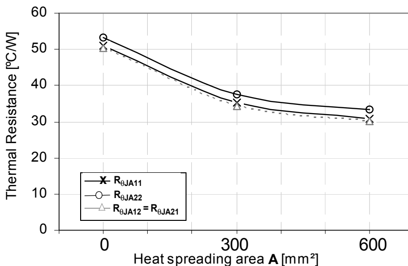
Figure 32. Device on Thermal Test Board R_{\theta JA}
