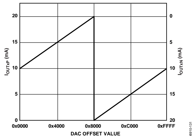
Figure 72. DAC Output Currents vs. DC Offset Value
