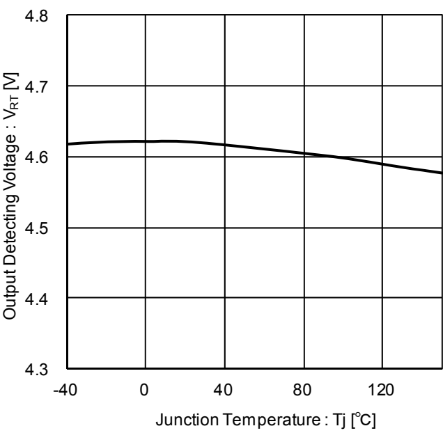
Figure 16. Output Detecting Voltage vs Temperature ( R_O: 10\text{ k}\Omega pull-up to V_O )
