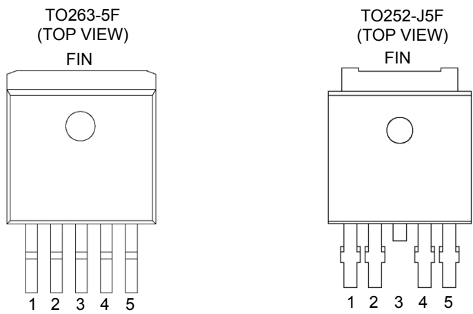
Figure 3. Pin configurations
