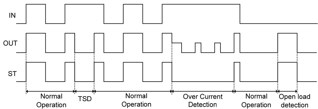
Figure 38. Timing Chart
