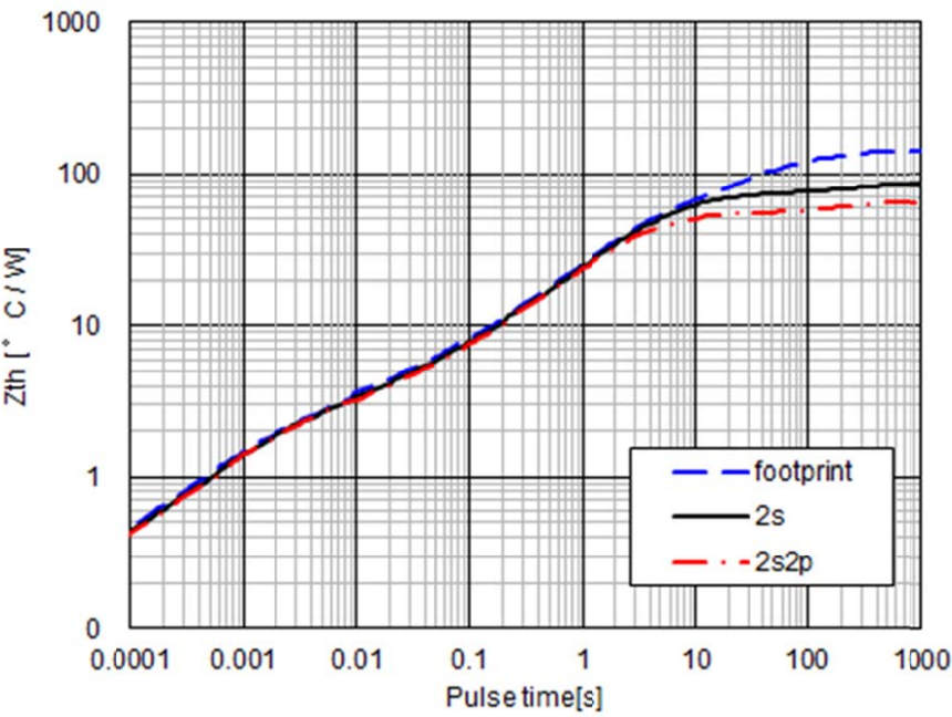
Figure 7. Thermal Resistance
