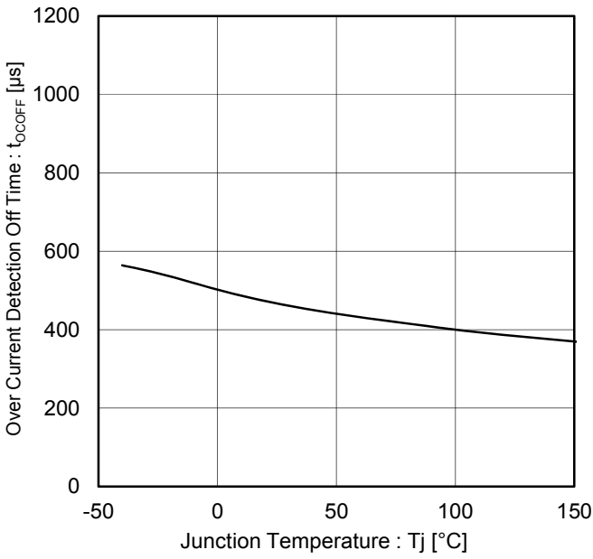
Figure 24. Overcurrent Detection Off Time vs. Temperature
