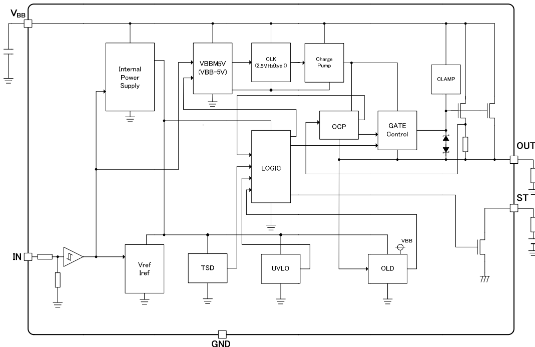
Figure 1. Block Diagram
