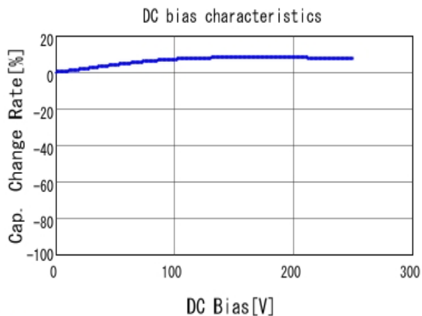
■ DE1E3KX102MN4AN01F C-DC bias capchange, 20.0degC, AC1
