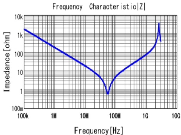
■ DE1E3KX102MN4AN01F |Z| DC0V, 20degC
