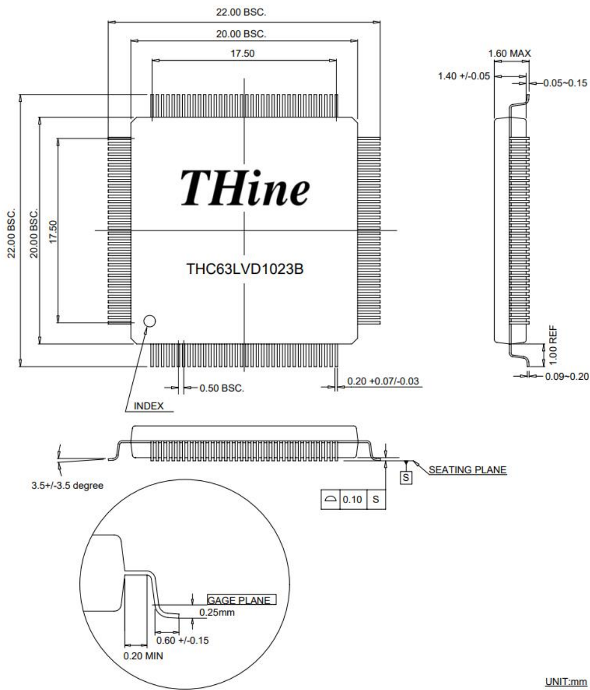
Figure 19. Package Diagram
