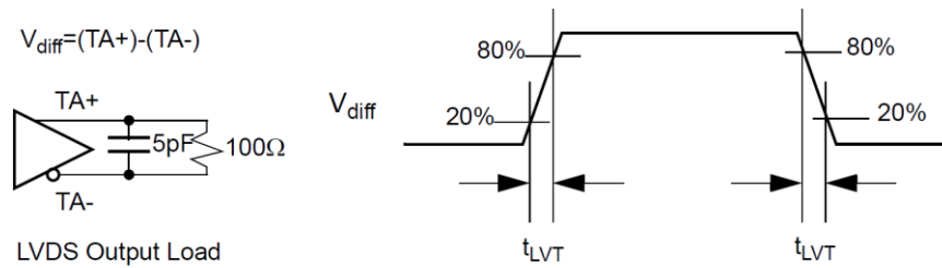
Figure 13. LVDS Output Load and Transition Time
