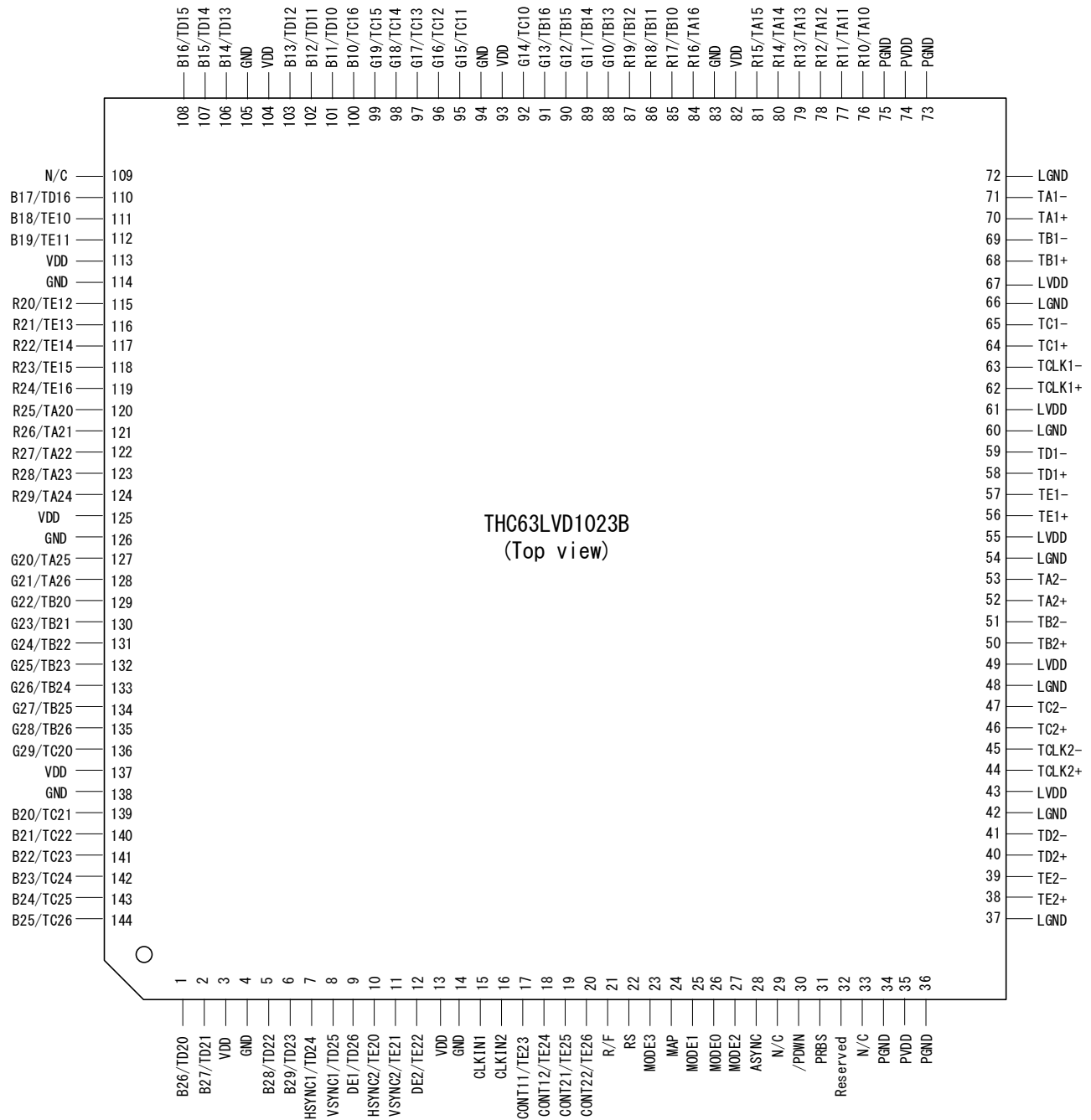
Figure 2. Pin Diagram
