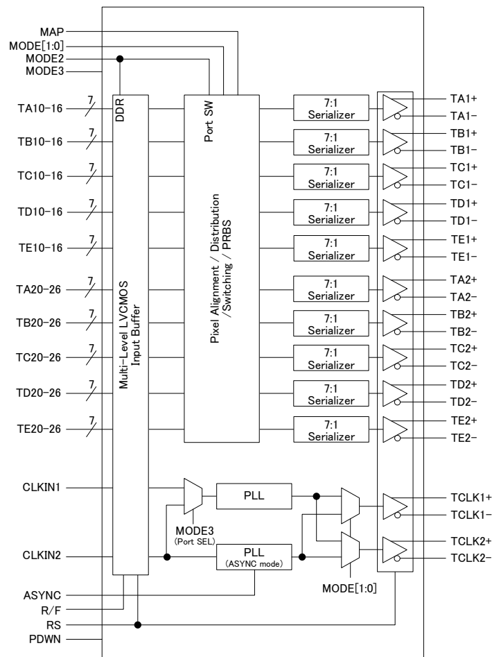
Figure 1. Block Diagram
