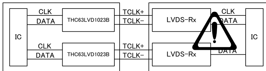
Figure 18. Asynchronous Use
