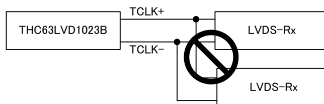
Figure 17. Multi Drop Connection
