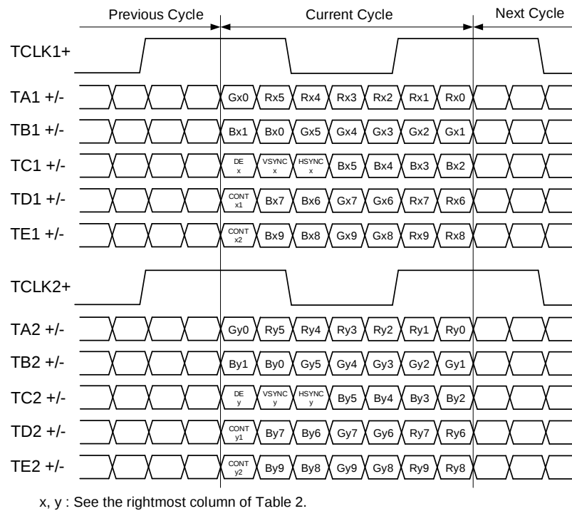
Figure 6. LVCMOS Inputs Mapped to LVDS Outputs (ASYNC=L, MAP=V IM3 )
