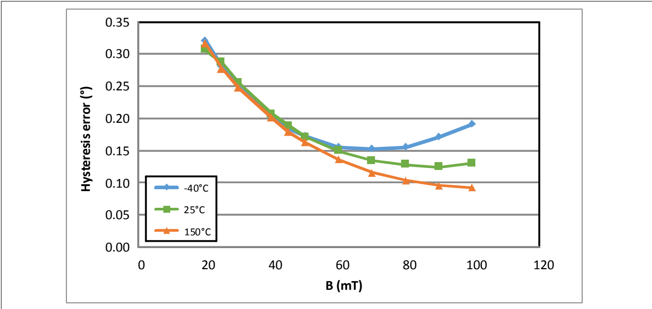
Figure 11 Typical hysteresis
