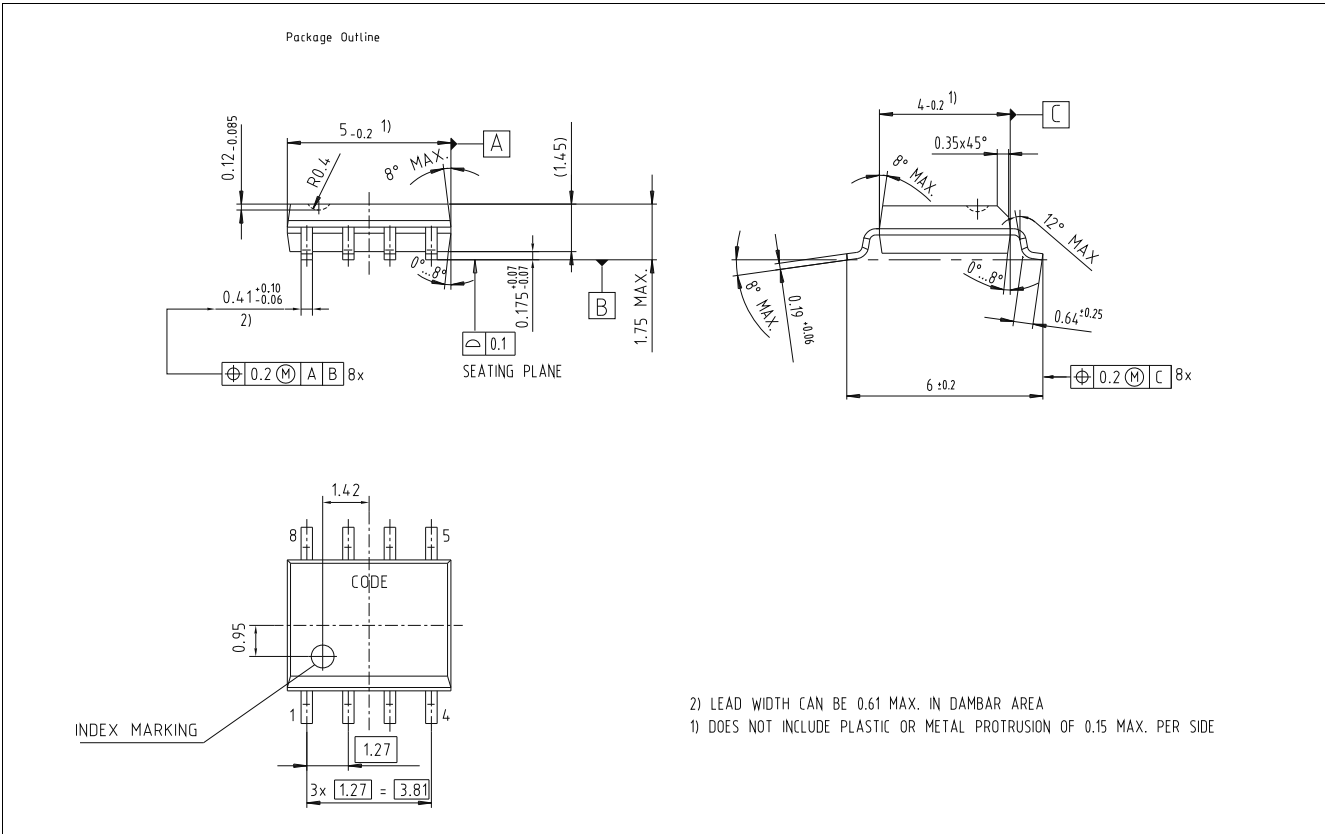
Figure 12 Package outline
