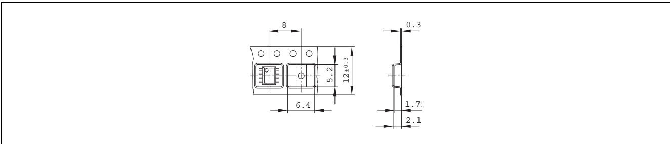
Figure 14 Packing
