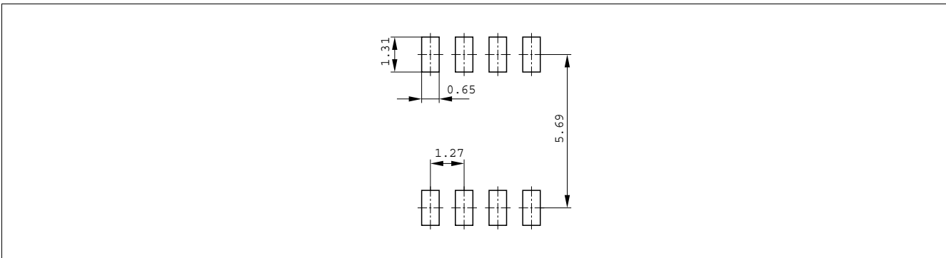
Figure 13 Footprint
