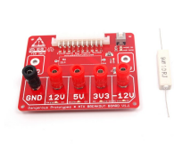
ATX breakout board bench power supply
