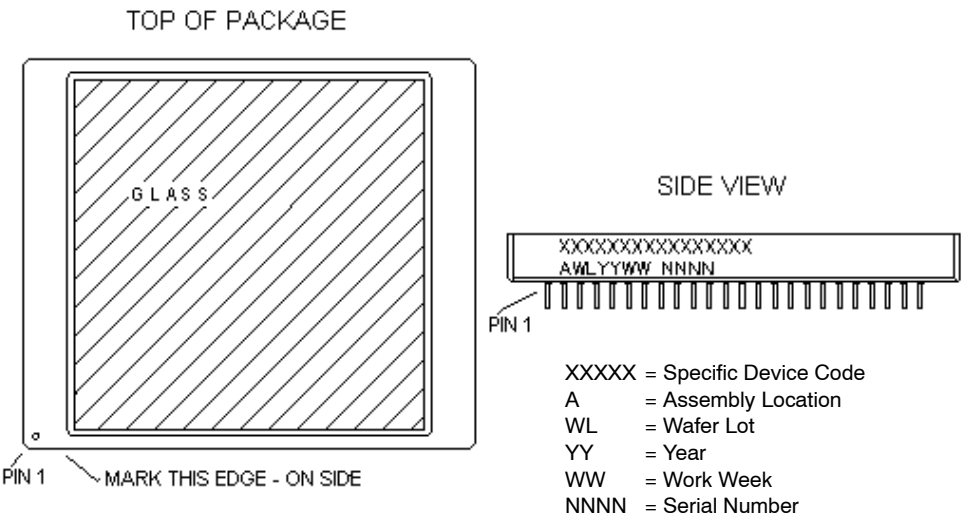
Figure 2. Marking Diagram
