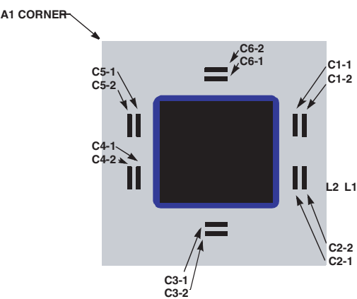
Figure 12-8. Substrate Capacitors for the PC7410
