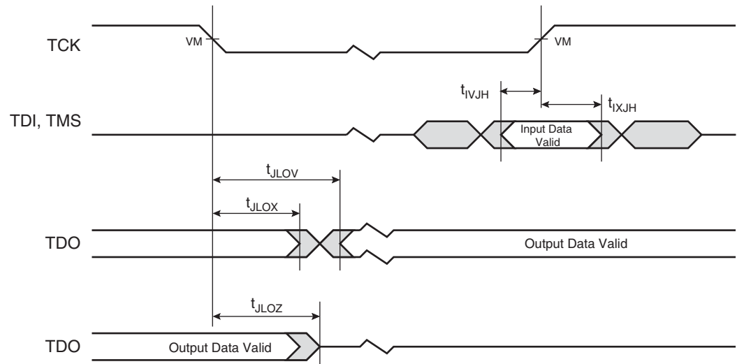
Figure 9-13. Test Access Port Timing Diagram
