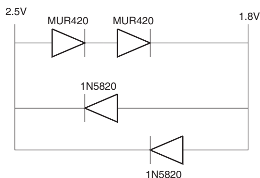
Figure 14-3. Example Voltage Sequencing Circuits
