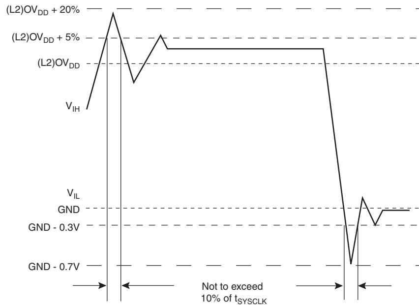
Figure 6-1. Overshoot/Undershoot Voltage
