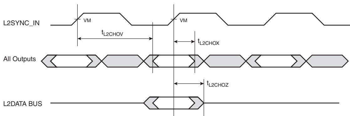
Figure 9-7. L2 Bus Output Timing Diagram
