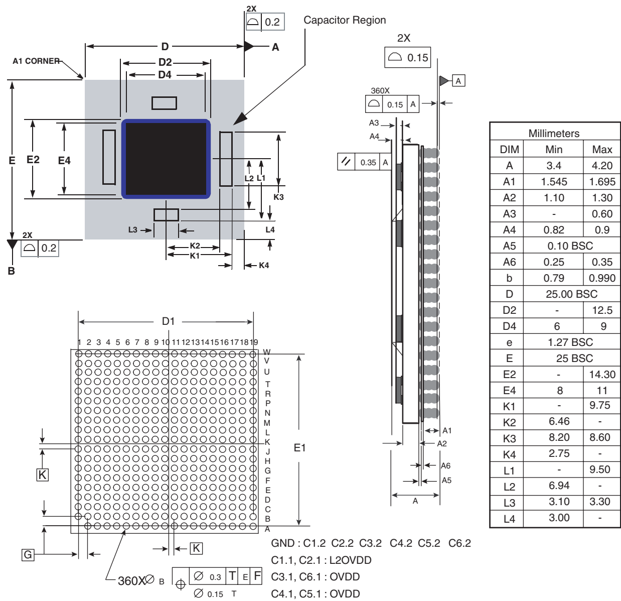
Figure 12-7. Mechanical Dimensions and Bottom Surface Nomenclature of the 360-column CI-CGA Package
