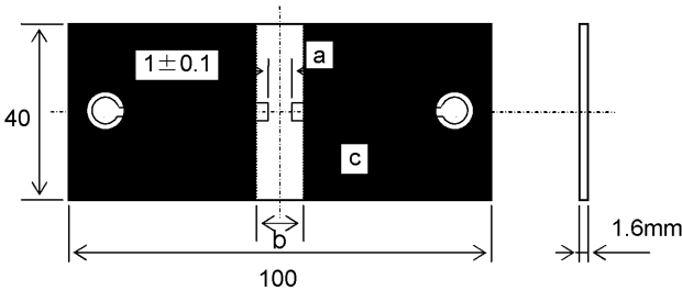
Fig.3 Test Board
