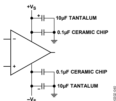
Figure 40. Recommended Power Supply Bypass
