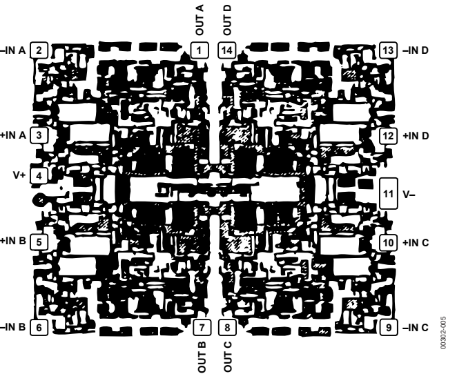
Figure 5. 0.111 Inch × 0.100 Inch DIE Size, 11,100 sq. mils, Substrate Connected to V+, 165 Transistors
