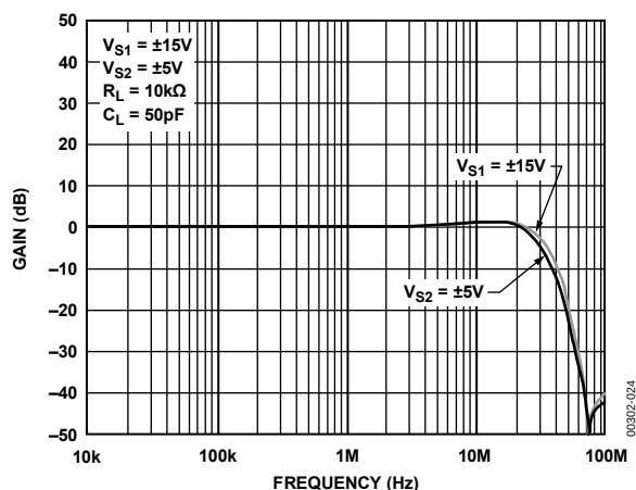
Figure 24. Noninverting Gain vs. Supply Voltage
