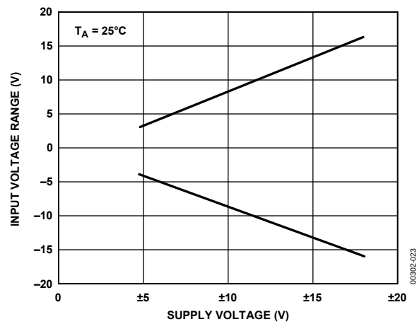
Figure 23. Input Voltage Range vs. Supply Voltage
