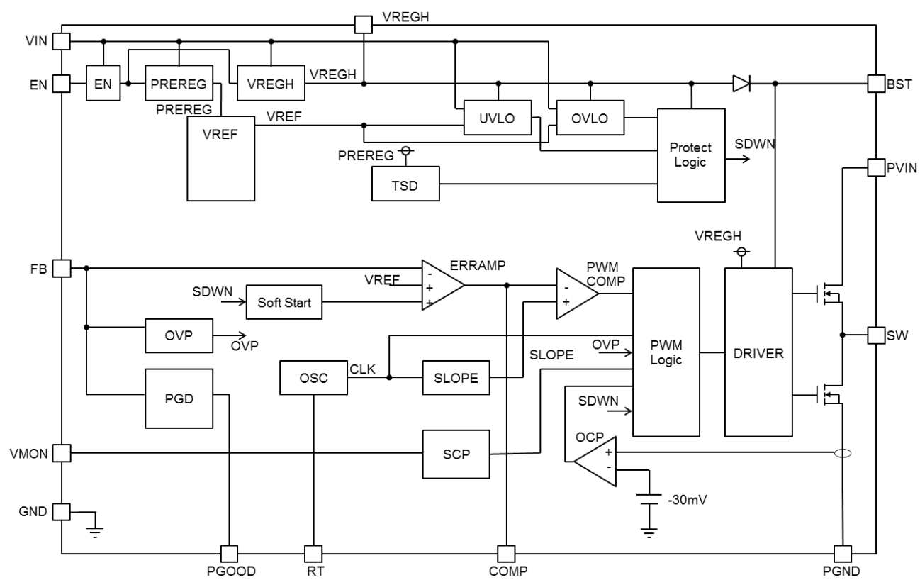
Figure 3. Block Diagram
