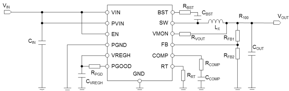
Figure 1. Application Circuit
