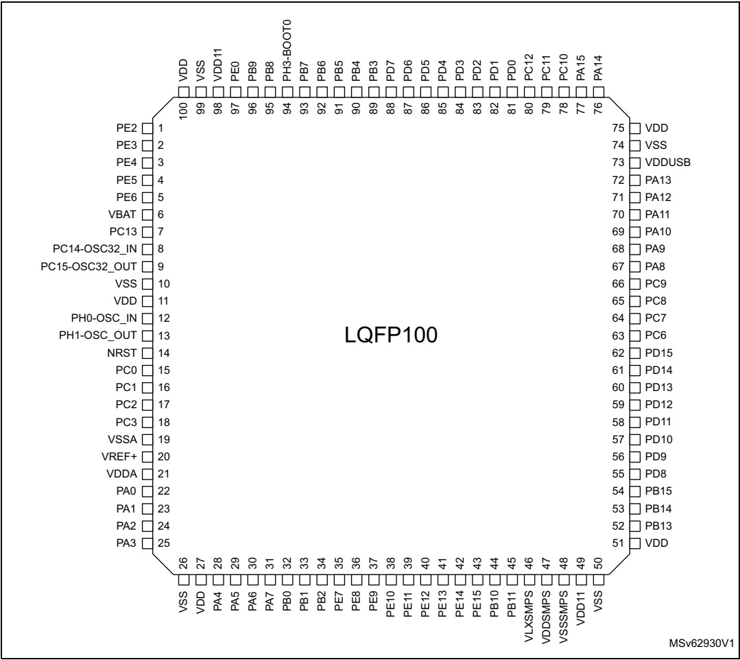
Figure 14. LQFP100_SMPS pinout
