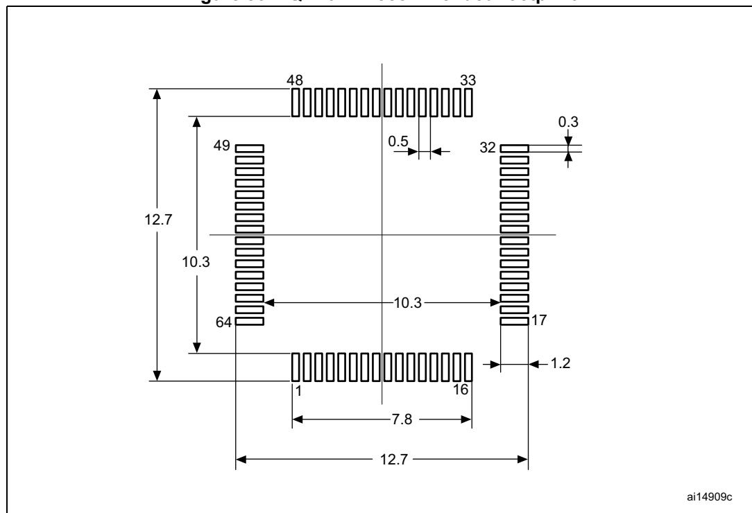
Figure 86. LQFP64 - Recommended footprint
