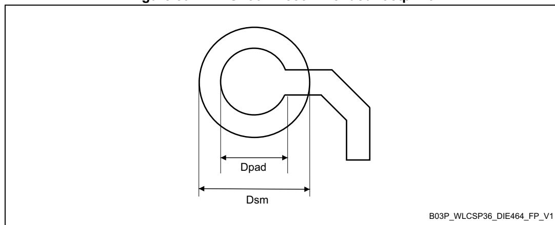
Figure 89. WLCSP90 - Recommended footprint
