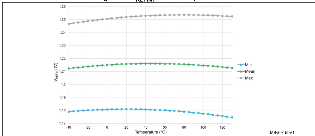
Figure 27. V_{\text{REFINT}} versus temperature
