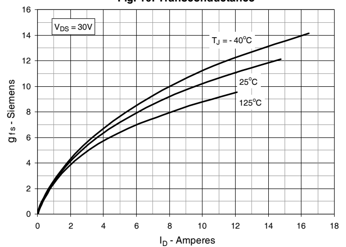
Fig. 10. Transconductance
