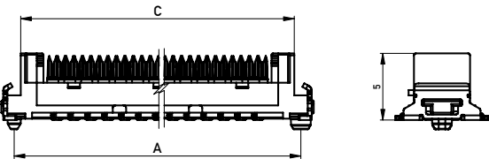
Board-on Connectors
