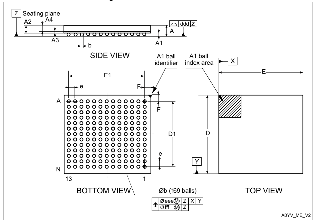
Figure 75. UFBGA169 - Outline
