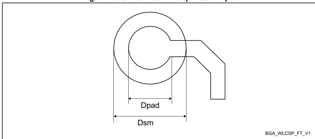
Figure 76. UFBGA169 - Footprint example
