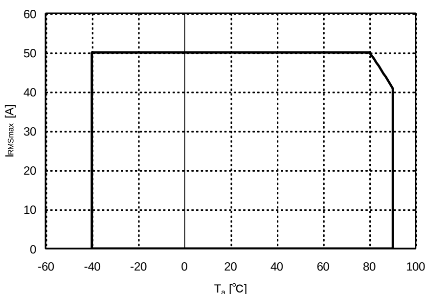
Figure 4. Primary current derating curve of CQ-206A
