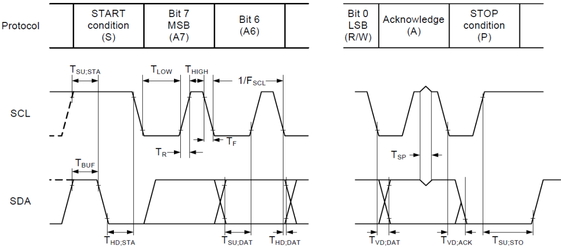
Figure 1: Timing Diagram
