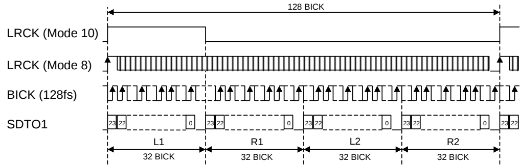
Figure 16. Mode 8/10 Timing (TDM128 mode, MSB justified)
