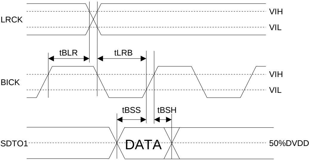
Figure 7. Audio Interface Timing (Slave mode, TDM0 pin = “H”, TDM1 pin = “H”, 108KHz < fs ≤ 216KHz)
