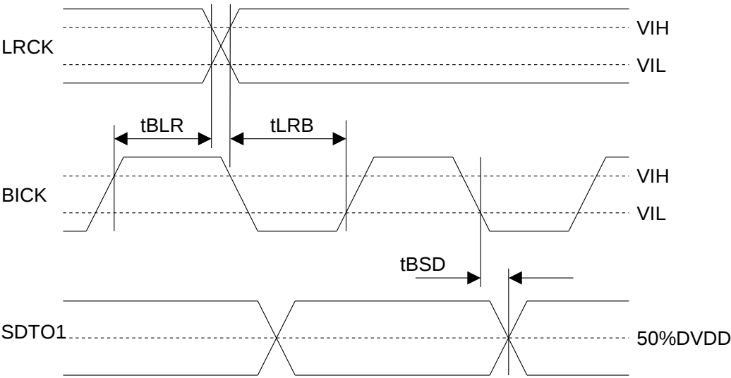
Figure 6. Audio Interface Timing (Slave mode, TDM0 pin = “H”, TDM1 pin = “H”, 8KHz ≤ fs < 108KHz)
