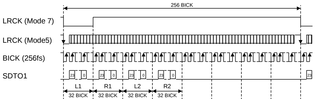
Figure 15. Mode 5/7 Timing (TDM256 mode, I 2 S Compatible)
