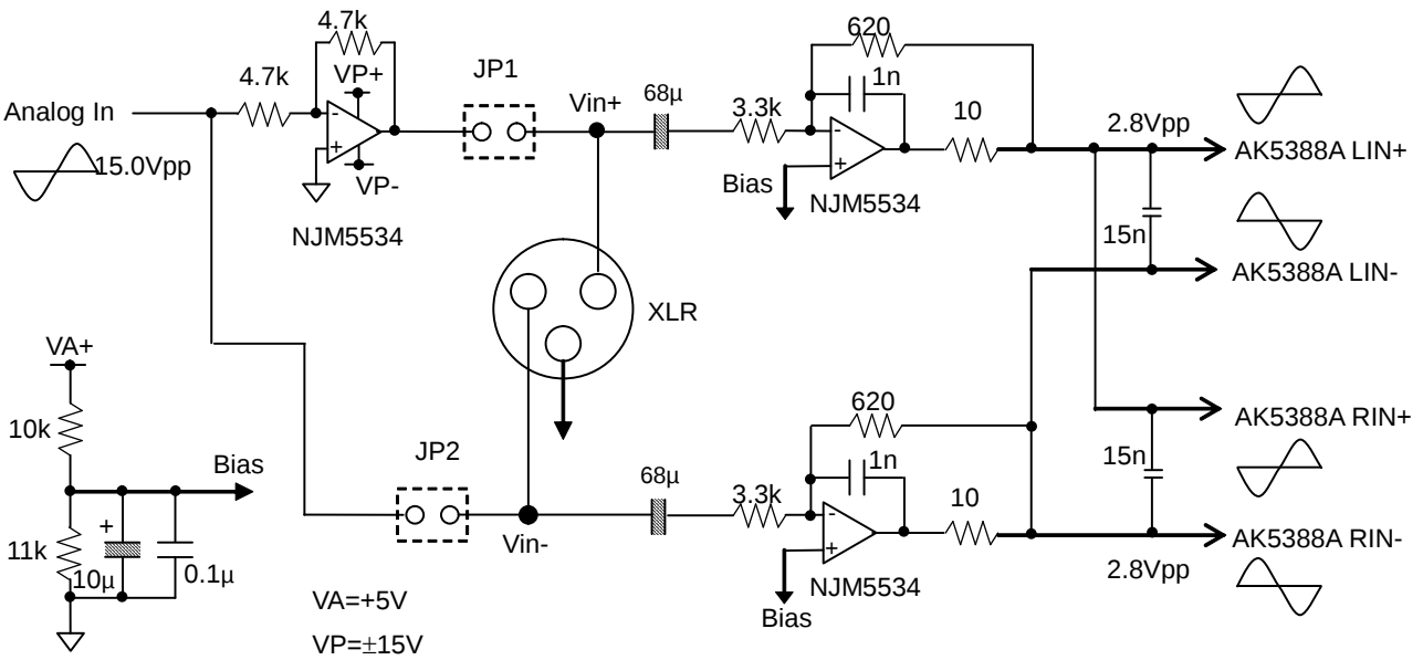
Figure 26 shows an input buffer circuit example in Mono mode. (1 st order HPF; f_c=0.70\text{Hz} , 2 nd order LPF; f_c=351\text{kHz} , gain=-14.5dB).
