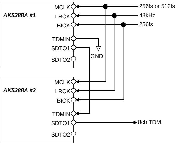
Figure 19. Cascade TDM Connection Diagram
