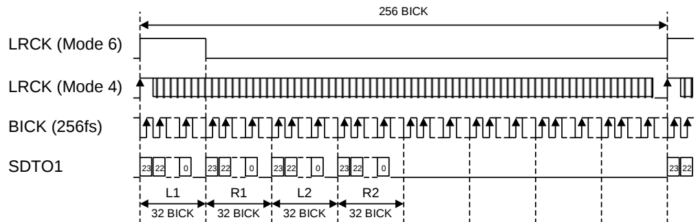
Figure 14. Mode 4/6 Timing (TDM256 mode, MSB justified)
