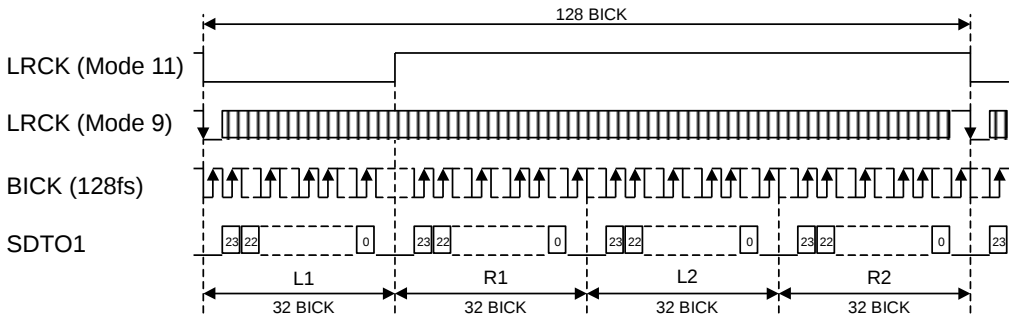
Figure 17. Mode 9/11 Timing (TDM128 mode, I 2 S Compatible)
