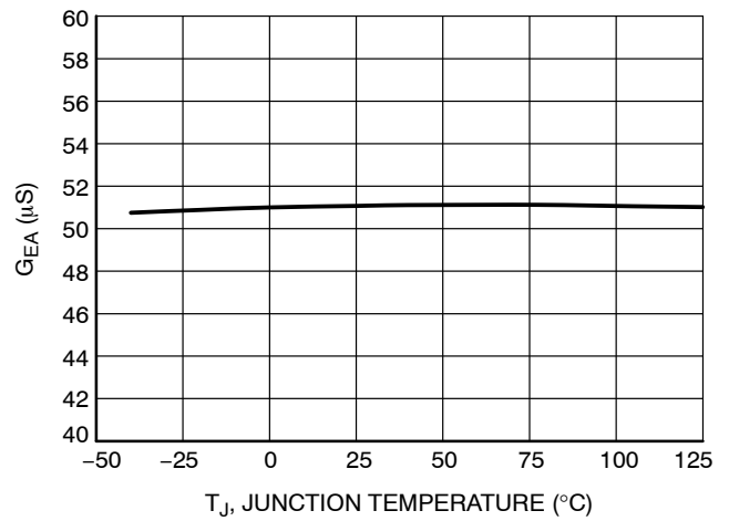
Figure 12. G EA vs. Junction Temperature
