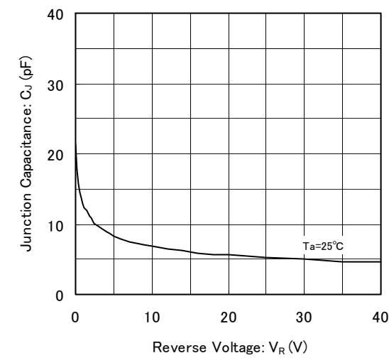
(3) Junction Capacitance vs. Reverse Voltage
