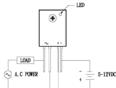
Fig.8 WIRING DIAGRAM
