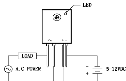
Fig.8 WIRING DIAGRAM
