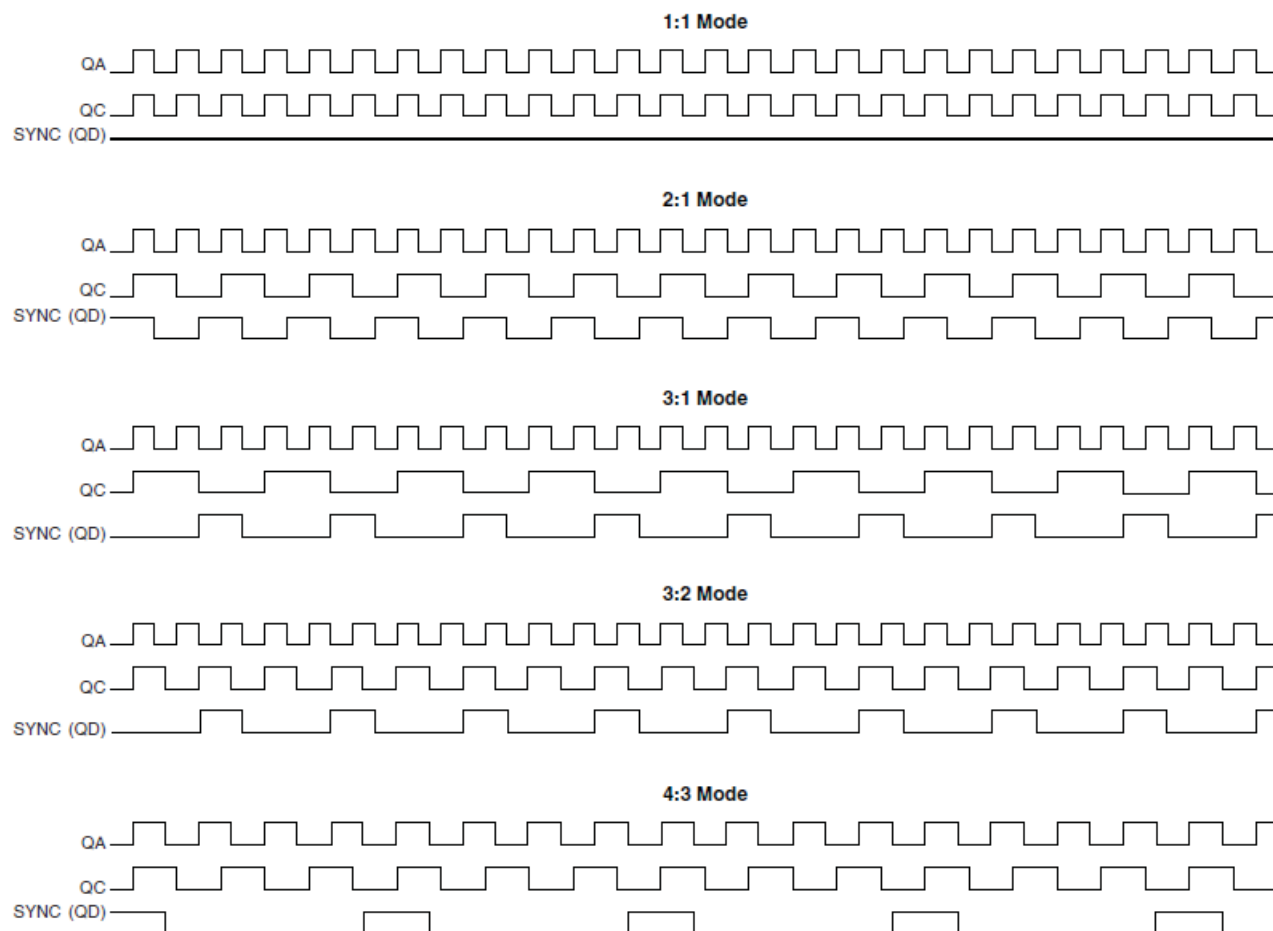
FIGURE 1. TIMING DIAGRAMS
