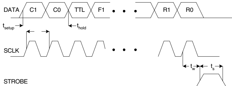
Figure 2. Timing Diagram for Programming the ICS307
