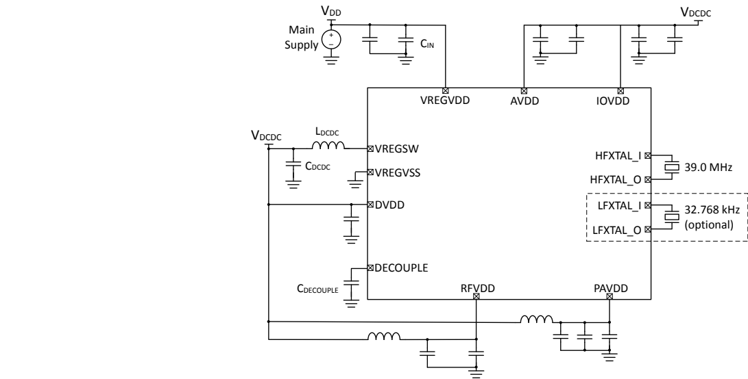
Figure 5.3. EFR32MG26 Typical Application Circuit: DCDC Configuration with PAVDD, RFVDD, AVDD, and IOVDD from DCDC output
