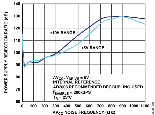
Figure 30. PSRR
