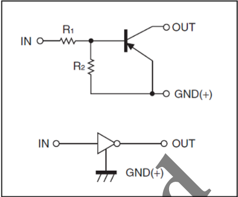
Equivalent Circuit
