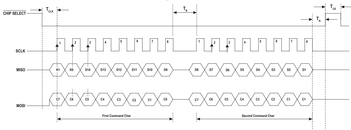
Figure 1 Timing Waveform
