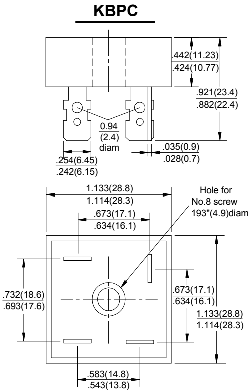
Dimensions in inches and (milimeters)
