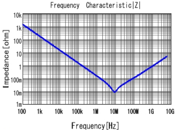
■ GRM033R60G155ME14 |Z| DC0V, 25degC
