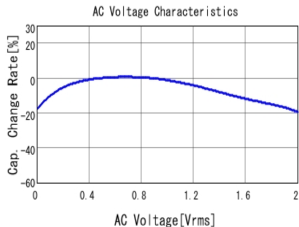
■ GRM033R60G155ME14 C-AC Voltage capchange, DC0V, 25.0d
