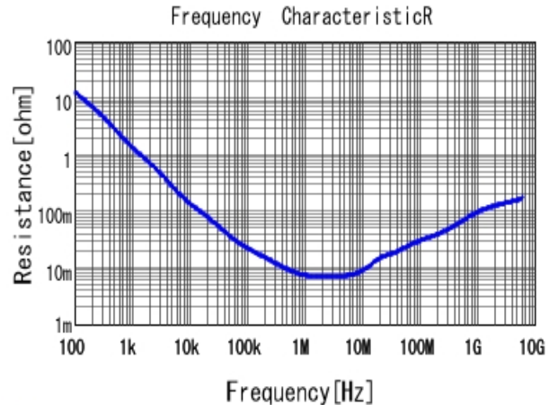
■ GRM033R60G155ME14 R DC0V, 25degC
