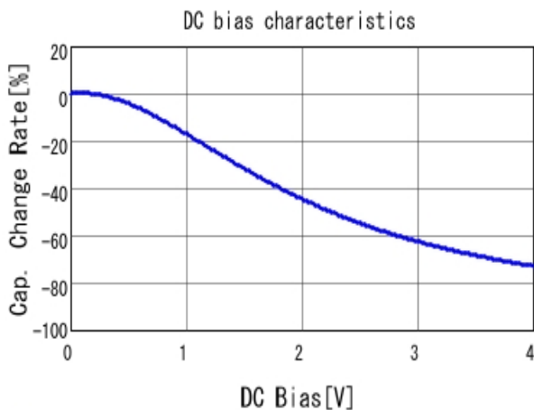
■ GRM033R60G155ME14 C-DC bias capchange, 25.0degC, AC0.
