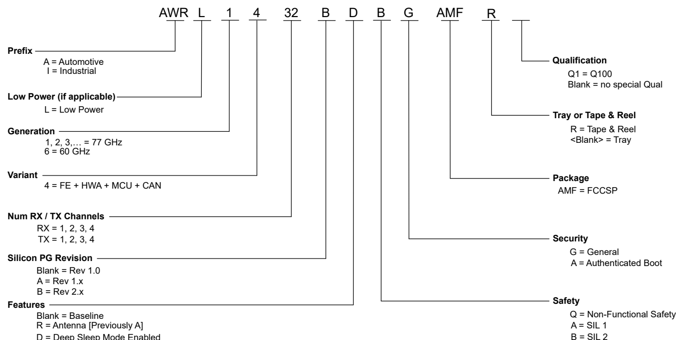
Figure 11-1. Device Nomenclature
