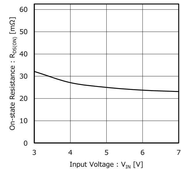
Figure 6. On-state Resistance vs Input Voltage
