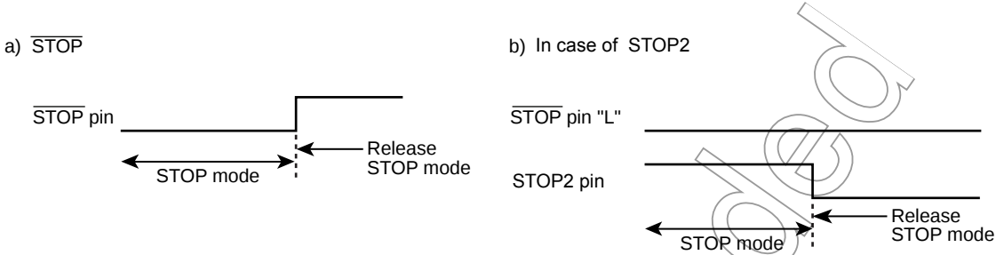
Figure 14-2 Priority of STOP pin and STOP2 pin
