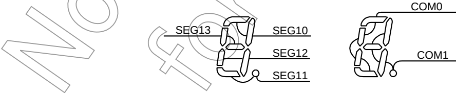
Figure 15-6 Example of COM, SEG Pin Connection
