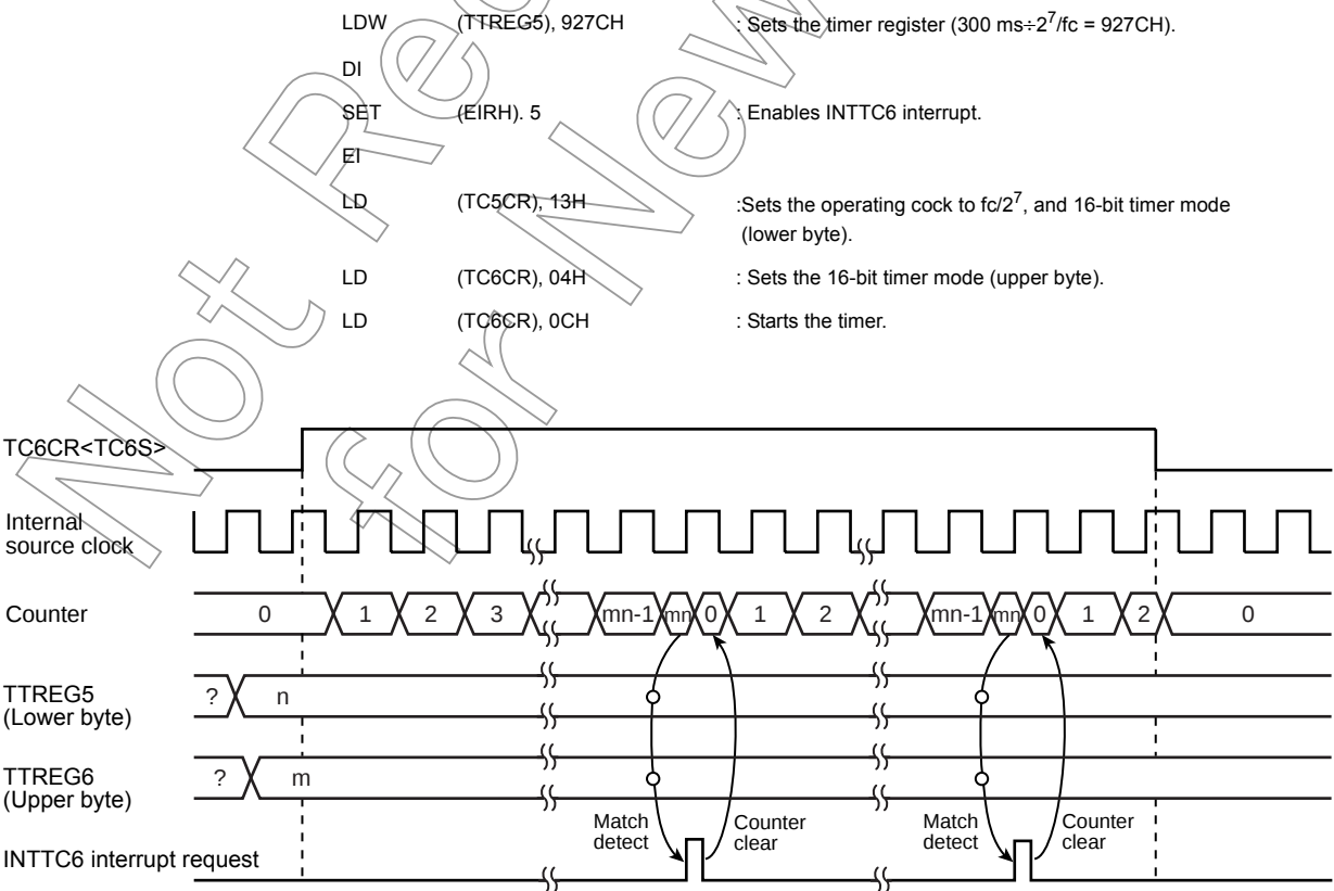
Figure 9-6 16-Bit Timer Mode Timing Chart (TC5 and TC6)
