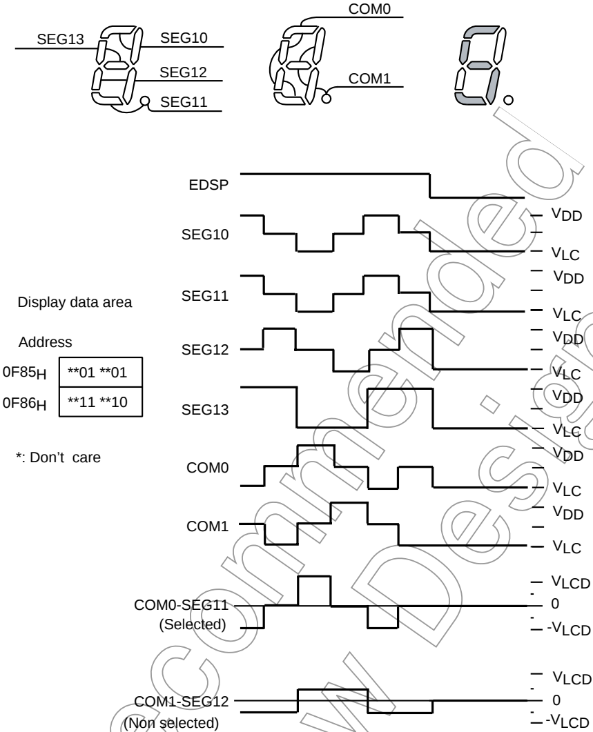
Figure 15-10 1/2 Duty (1/2 Bias) Drive
