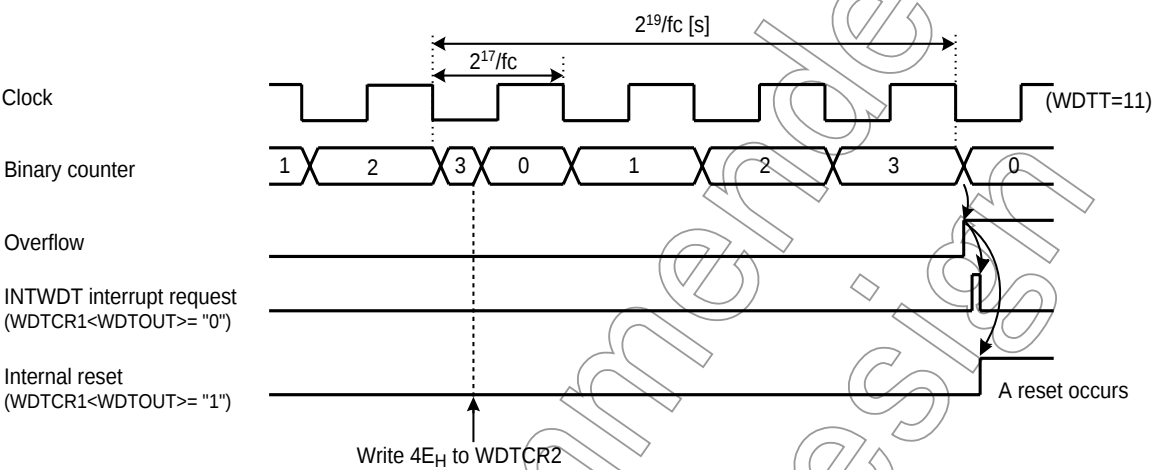
Figure 6-2 Watchdog Timer Interrupt
