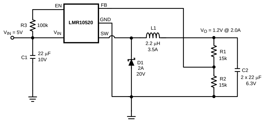
Figure 20. LMR10520x (1.6 MHz): V_{IN} = 5\text{ V} , V_{OUT} = 1.2\text{ V} at 2 A
