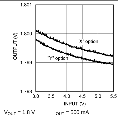
Figure 19. Line Regulation
