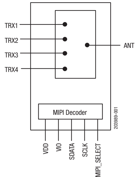
Figure 1. SKY13560-485LF Block Diagram
