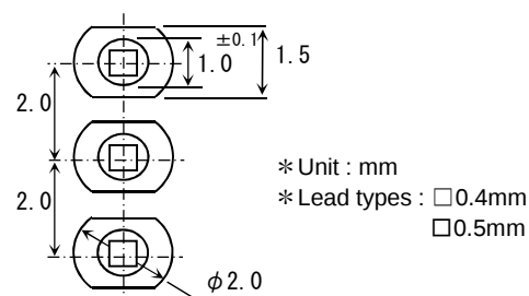
<3 lead pin type/2.0mm pitch>
