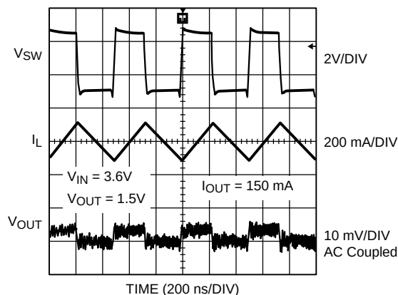
Figure 27. Typical PWM Operation
