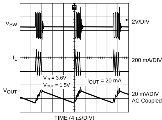
Figure 28. Typical PFM Operation
