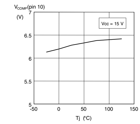
Figure 13. COMP voltage upper clamp level vs. Tj
