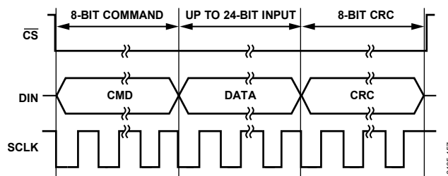
Figure 57. SPI Write Transaction with CRC
