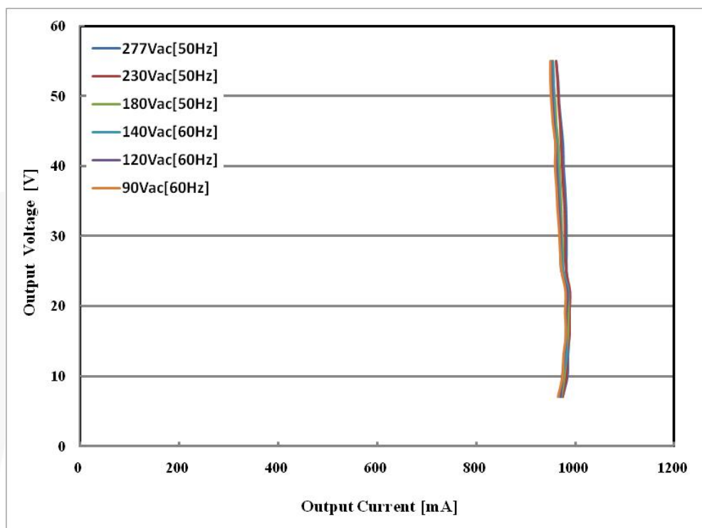
Figure 20. Constant-Current Regulation
