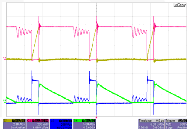
Figure 19. V_{IN} = 277 V_{AC} / 60 \text{ Hz} , [5.0 μs / div]
