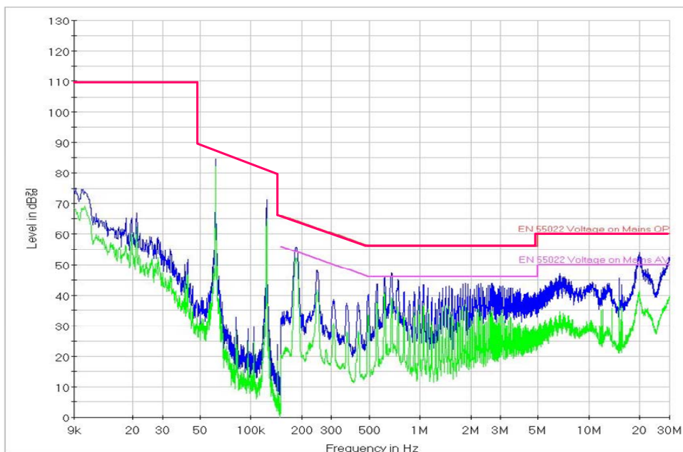
Figure 41. V_{IN} [220 V AC , Neutral]
