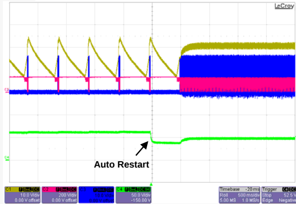
Figure 28. V_{IN} = 90 V_{AC} / 60 \text{ Hz} , [LED Restore]
