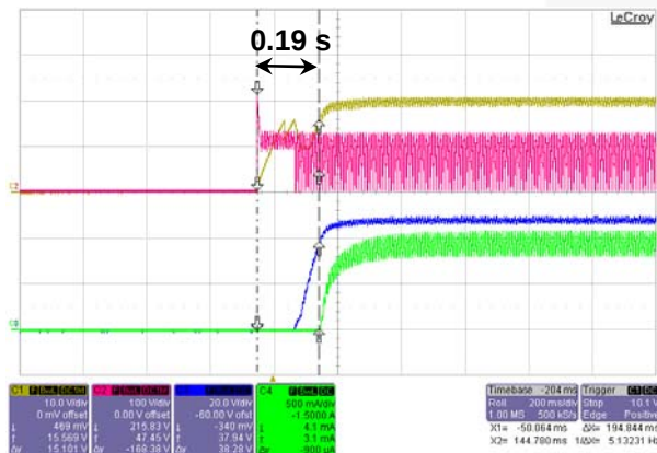
Figure 10. V_{IN} = 90\text{ V}_{AC} / 60\text{ Hz}
