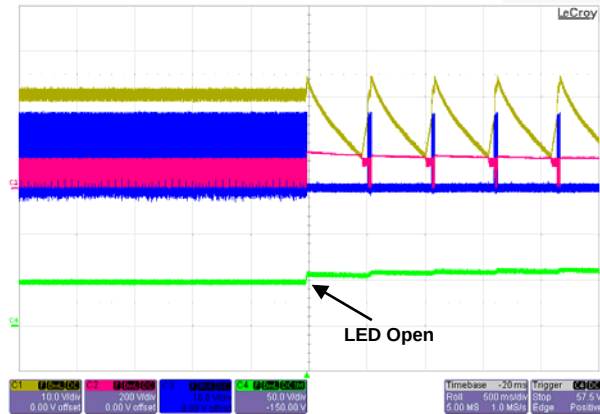
Figure 27. V_{IN} = 90 V_{AC} / 60 \text{ Hz} , [LED Short]
