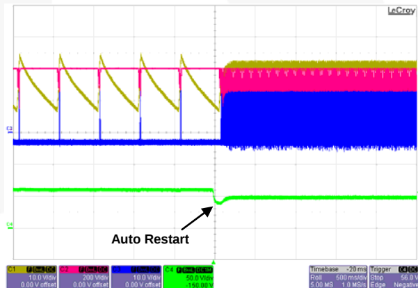
Figure 30. V_{IN} = 277 V_{AC} / 50 \text{ Hz} , [LED Restore]
