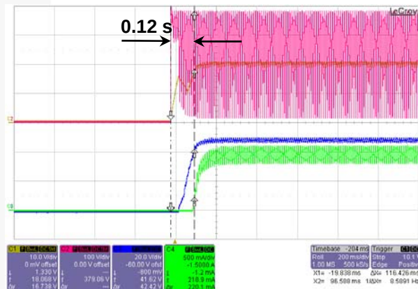
Figure 11. V_{IN} = 277 \text{ V}_{AC} / 50 \text{ Hz}
