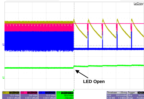
Figure 29. V_{IN} = 277 V_{AC} / 50 \text{ Hz} , [LED Short]
