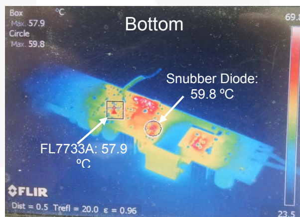
Figure 40. V_{IN} = 277 V_{AC} / 50 \text{ Hz}
