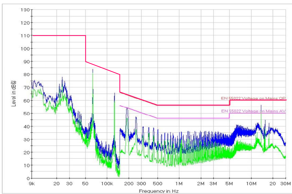
Figure 42. V_{IN} [110 V AC , Live]
