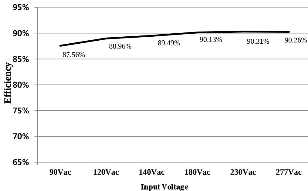
Figure 31. System Efficiency
