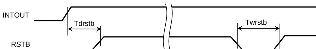
Fig. 4-9-2 RSTB timing 1
