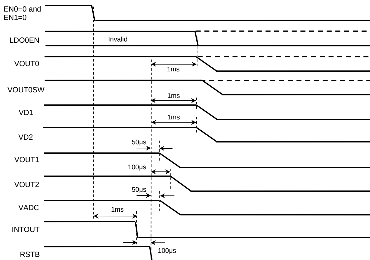
Fig. 4-7-4 Power down timing (with EN0/1 setting)
