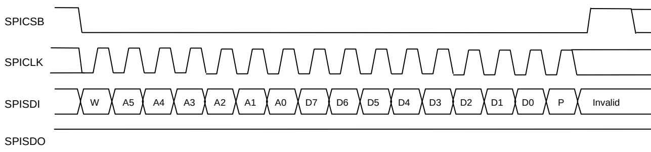
Fig. 4-2-1 SPI format (Write)
