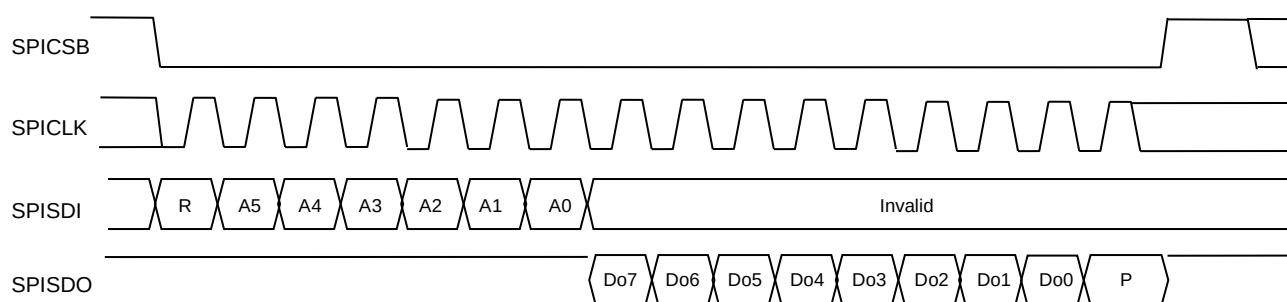
Fig. 4-2-2 SPI format (Read)
