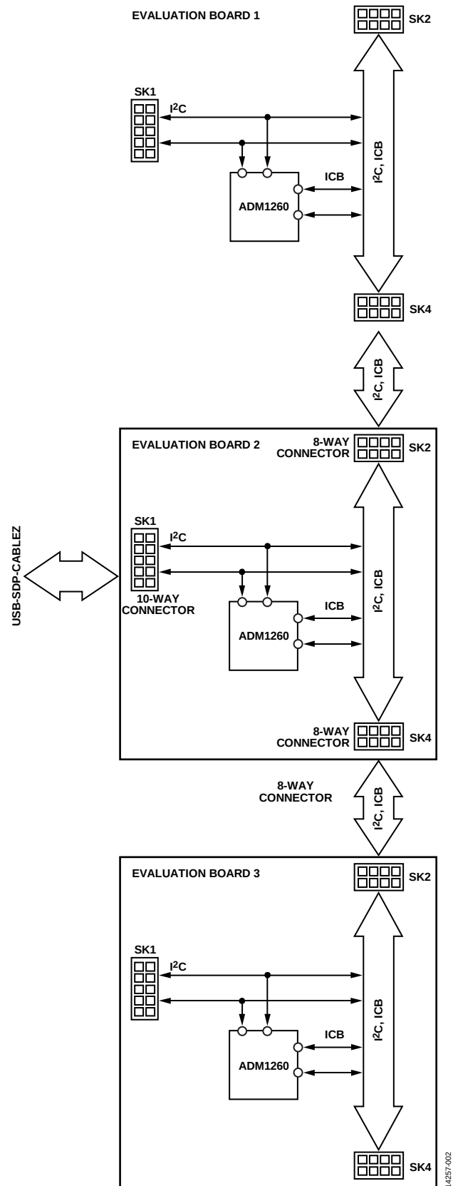
Figure 2. Multiple Boards Connection
