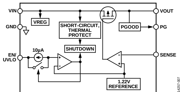
Figure 3. ADP7102 Functional Diagram
