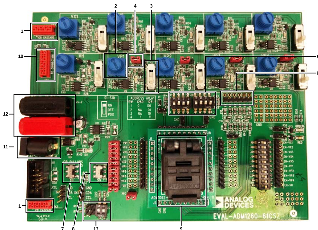
Figure 1. Evaluation Board Components
