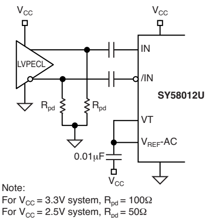
Figure 3b. AC-Coupled LVPECL Input Interface
