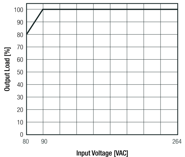
Line Derating
