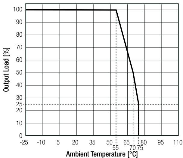
Derating Graph
