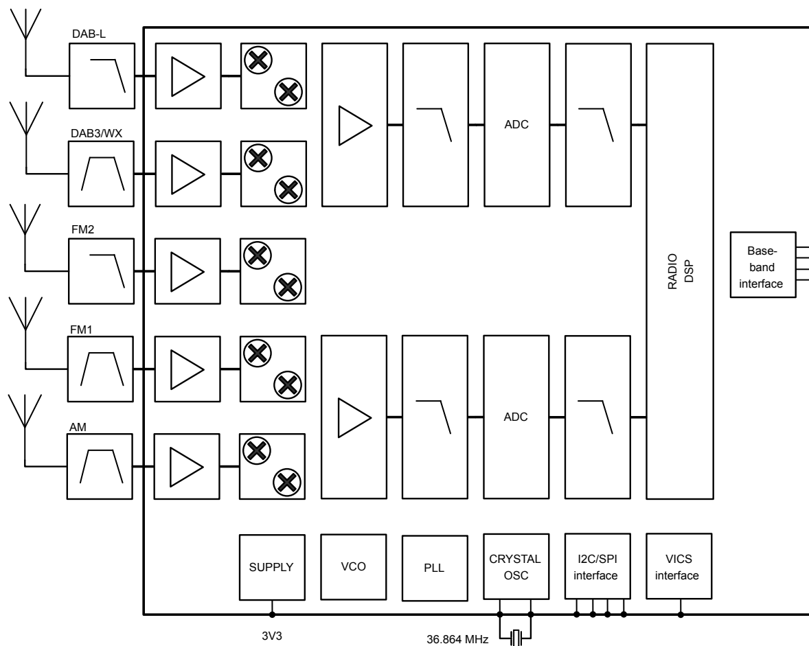
Figure 1. Block diagram
