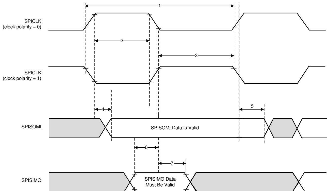
Figure 8-10. SPI Slave Mode External Timing (CLOCK PHASE = 0)
