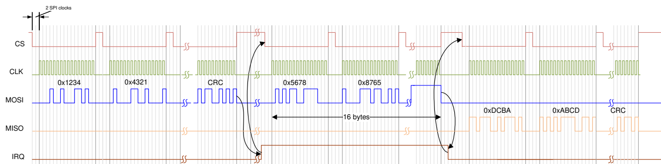
Figure 8-12. SPI Communication
