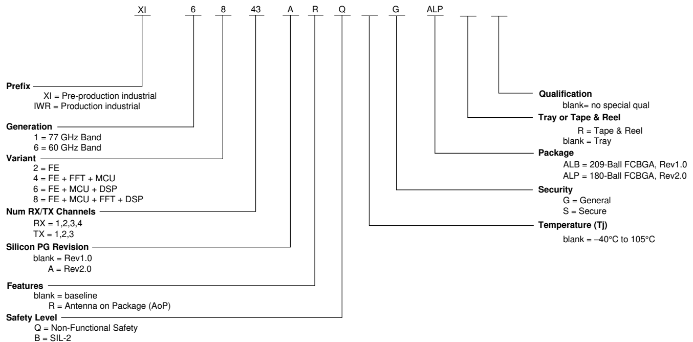
Figure 12-1. Device Nomenclature
