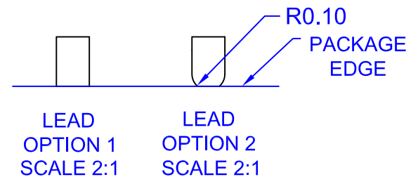
LEAD SHAPE AT PACKAGE EDGE
